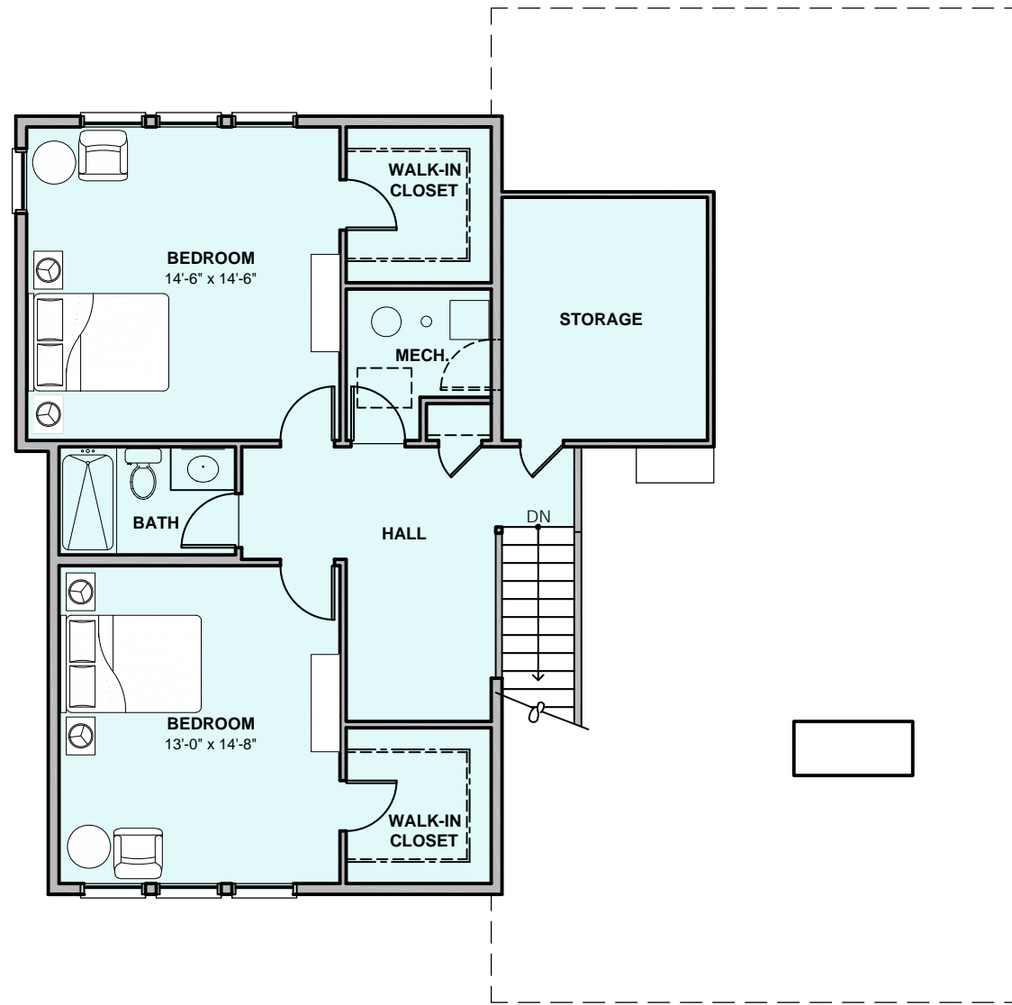
SECOND FLOOR PLAN 775 G.S.F.
