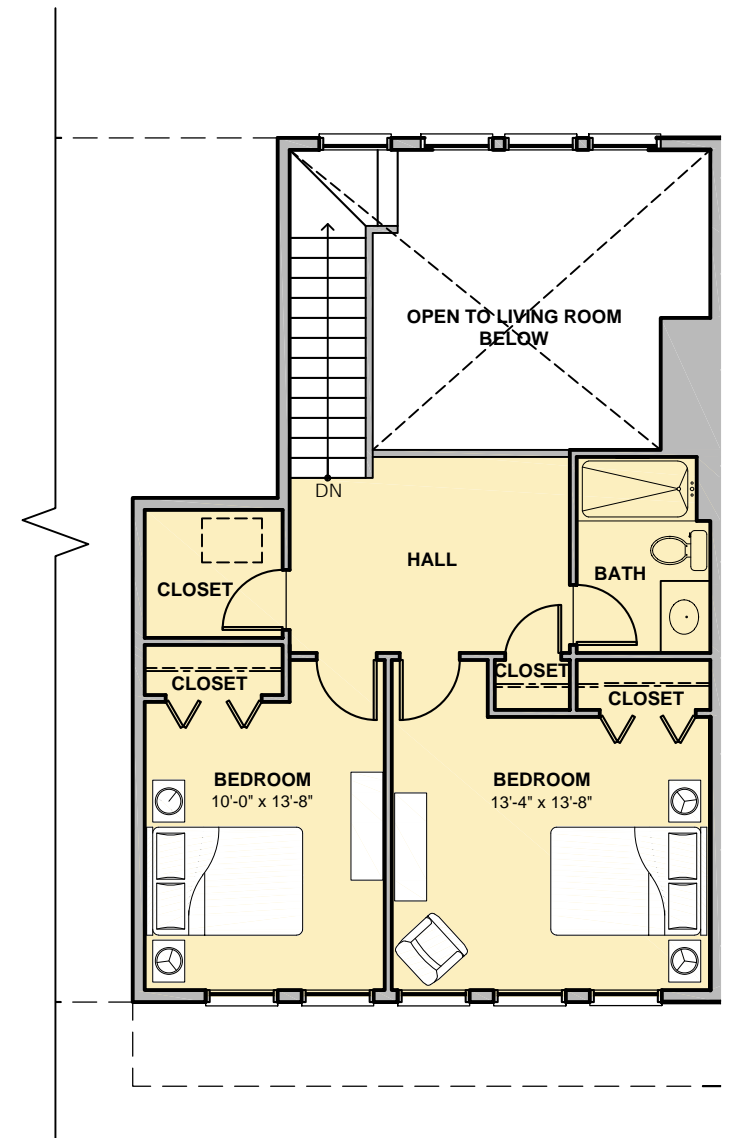
SECOND FLOOR PLAN 550 G.S.F.
