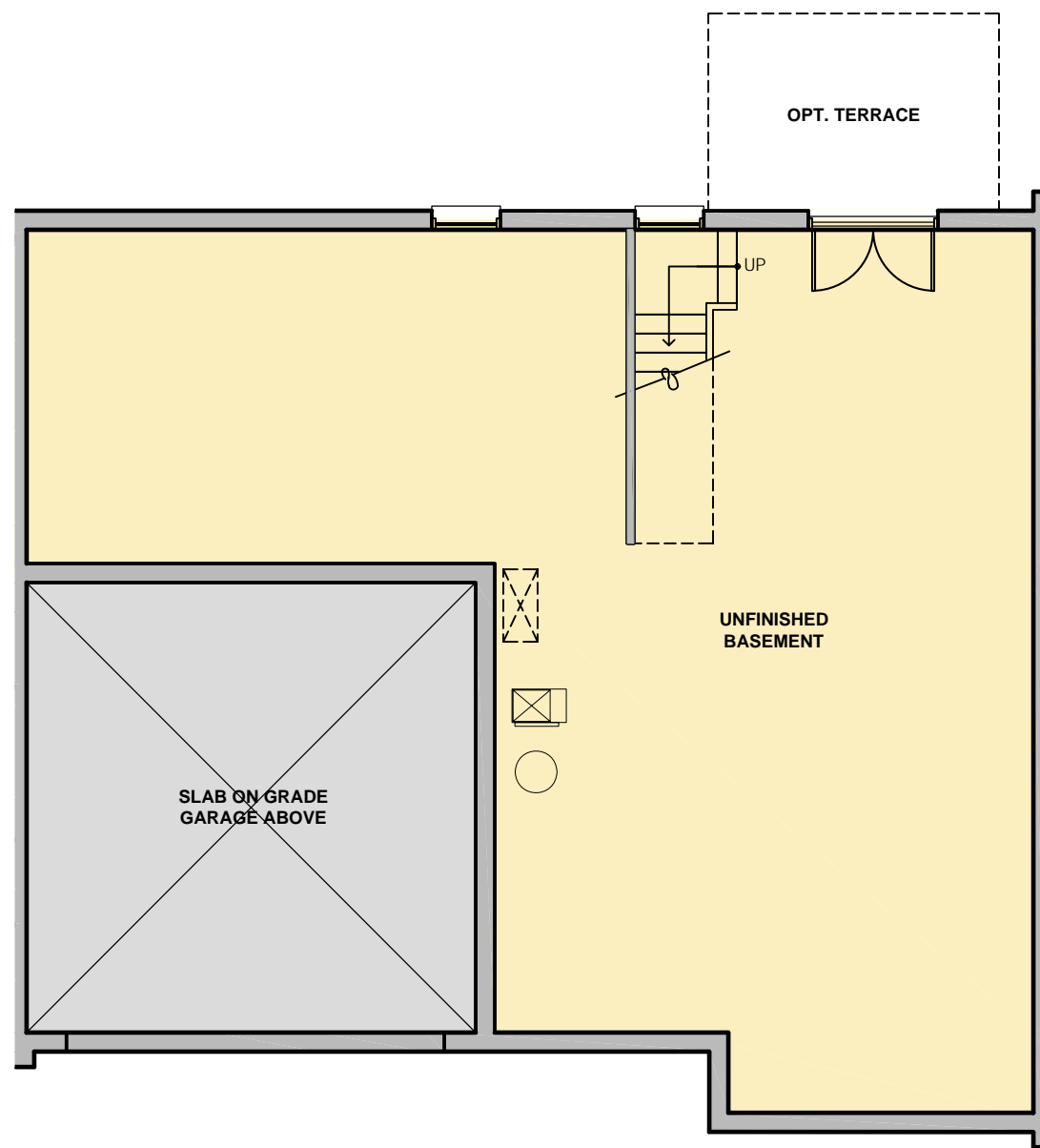
BASEMENT PLAN 1270 G.S.F.
