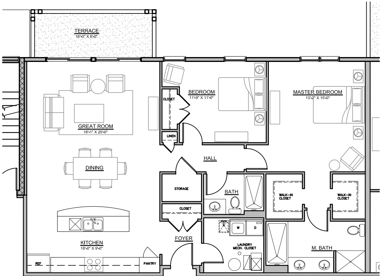
UNIT 202, 302, 402
