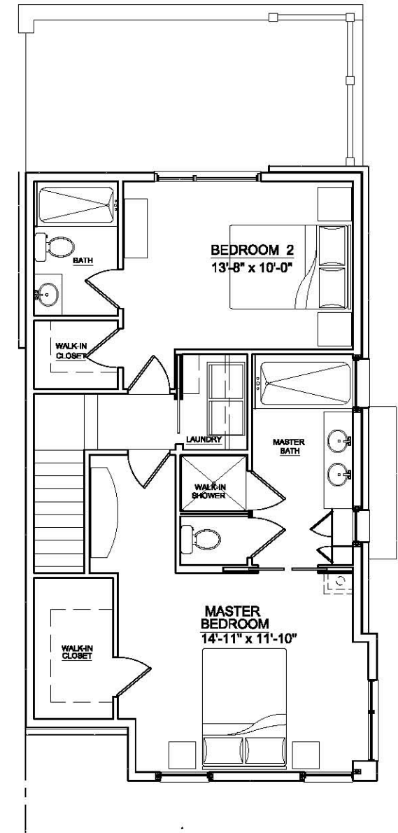
THIRD FLOOR PLAN 748 G.S.F. 0 1 2 4 6 8 FT.
