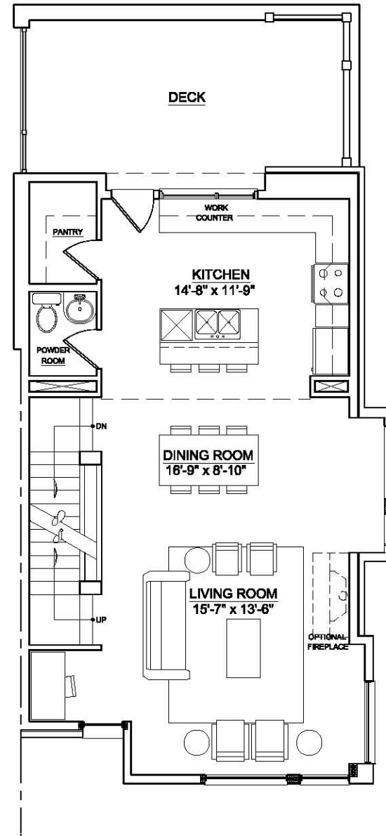
SECOND FLOOR PLAN 748 G.S.F. 0 1 2 4 6 8 FT.
