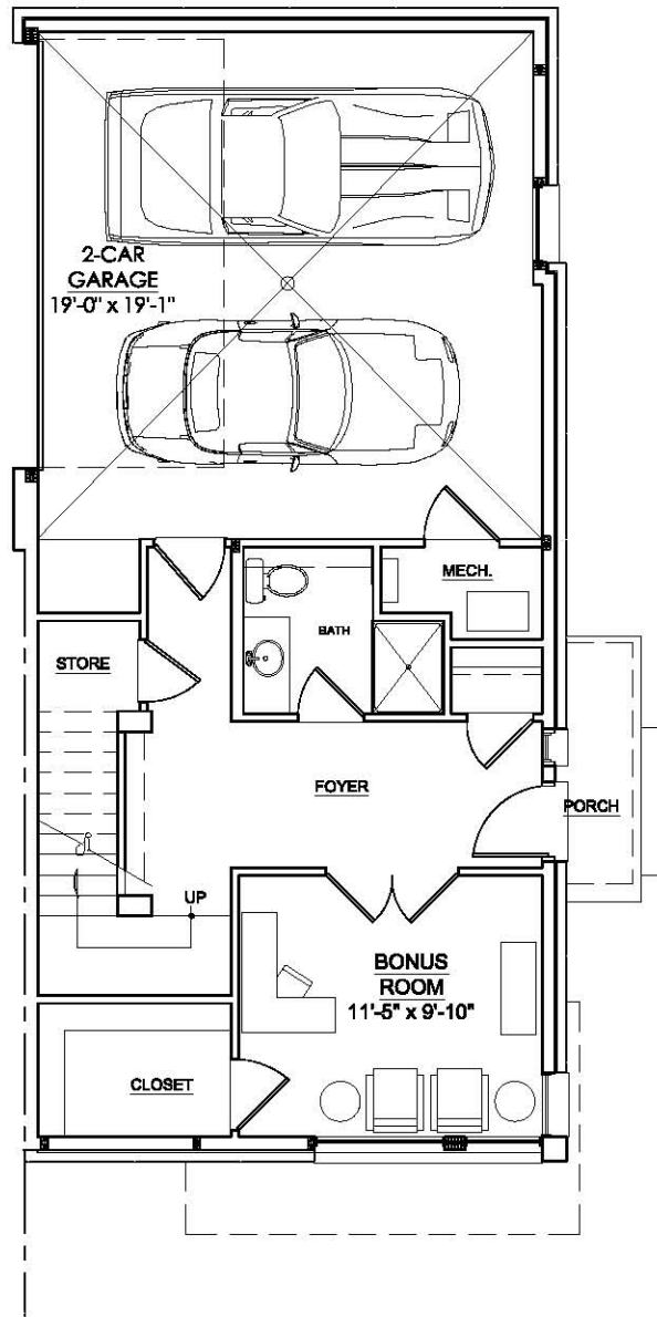
FIRST FLOOR PLAN 466 G.S.F. 0 1 2 4 6 8 FT.
